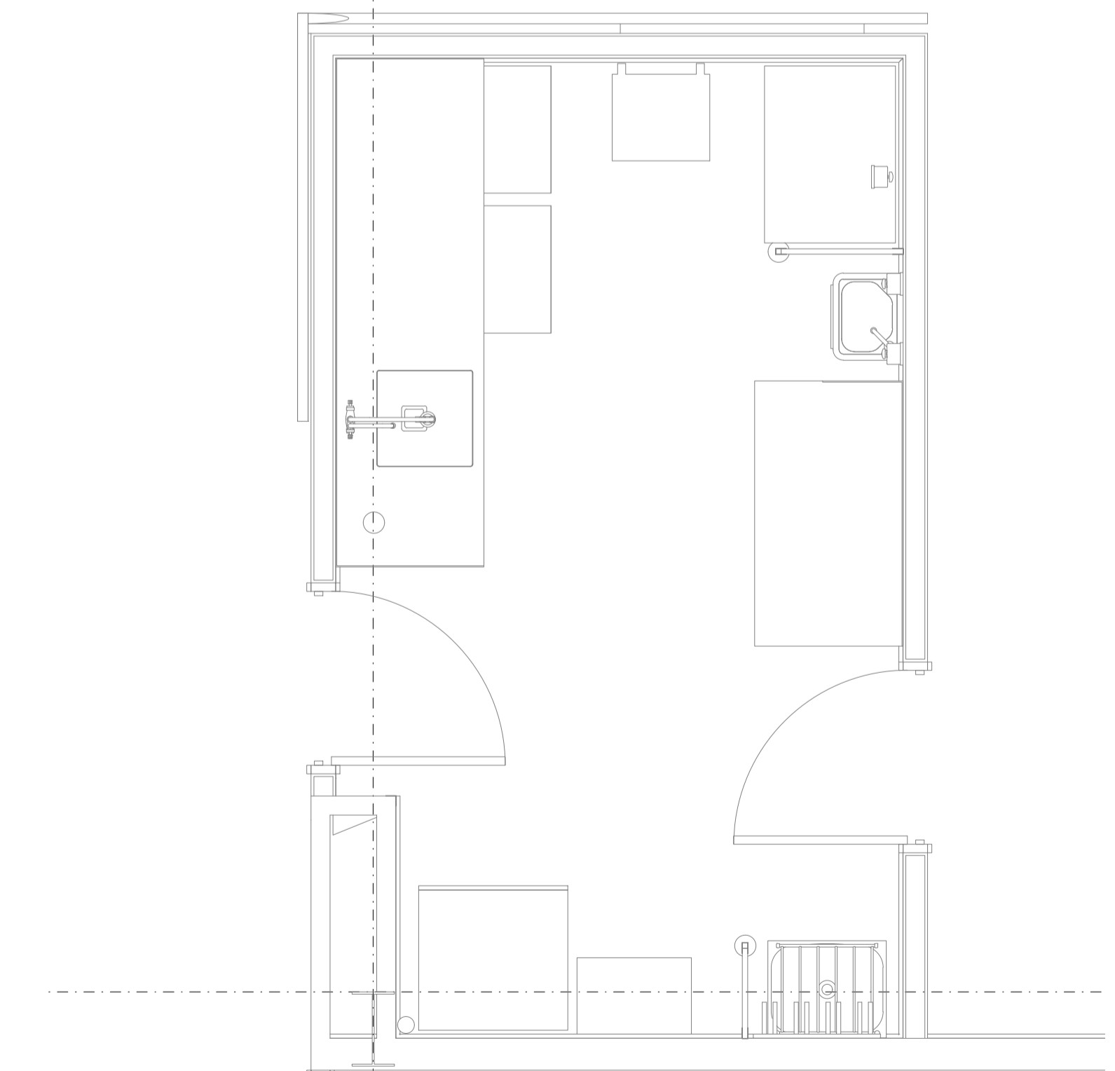
DETAIL C WASHUP ROOM FLOOR PLAN SCALE 1:25
